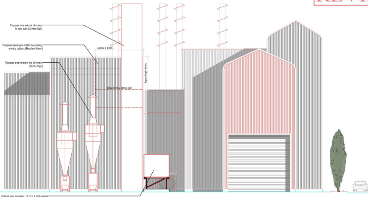
General Arrangement _Proposed South Elevation_ 1 : 100
