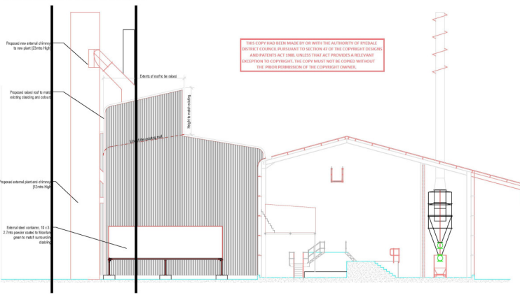
General Arrangement _Proposed West Elevation & Section A-A_ 1 : 100
